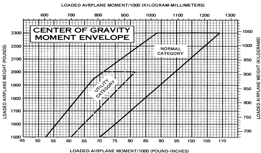
Figure 6-7. Center of Gravity Moment Envelope
